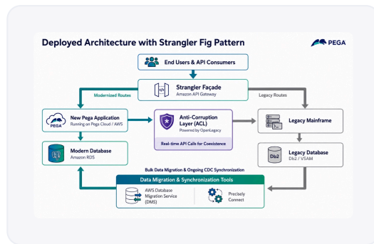
Figure 12: The Deployed Strangler Fig Architecture: A deployed architecture using the Strangler Fig Pattern to incrementally modernize a legacy mainframe system. A façade routes traffic, while an Anti-Corruption Layer and data migration tools ensure seamless coexistence and data synchronization between the new and old systems.
